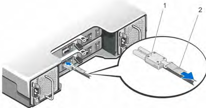
Figure 5. SAS Port and Cable Connections (Dell PowerVault MD1200 EMM)
